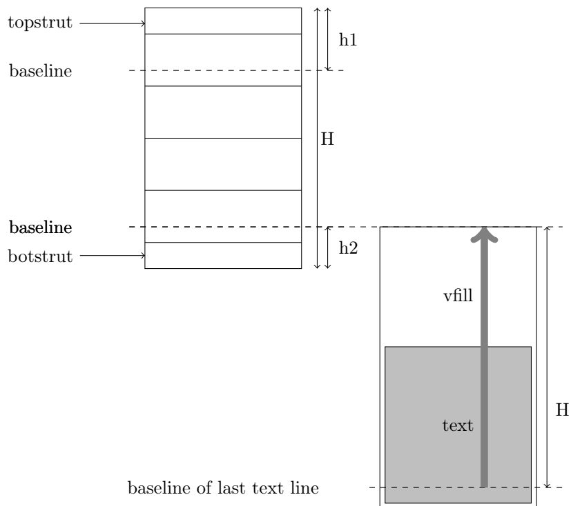
Figure 6: Case \langle nrows \rangle < 0 , \langle vpos \rangle = [\mathbf{b}]
