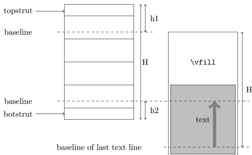
Figure 3: Case \langle n\text{rows} \rangle > 0 , \langle vpos \rangle = [\mathbf{b}]
